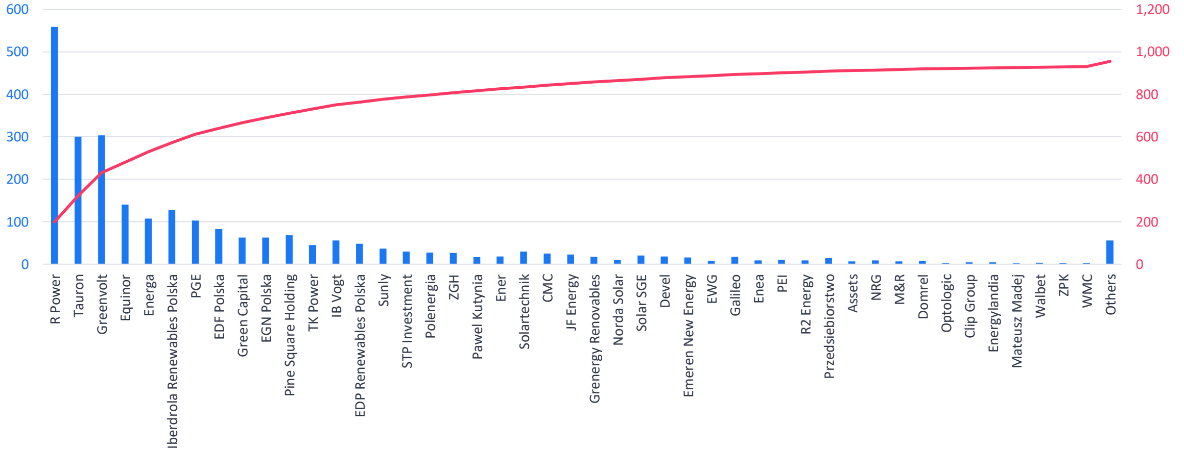
Cumulative amount of subsidies by NFOSiGW In M€
